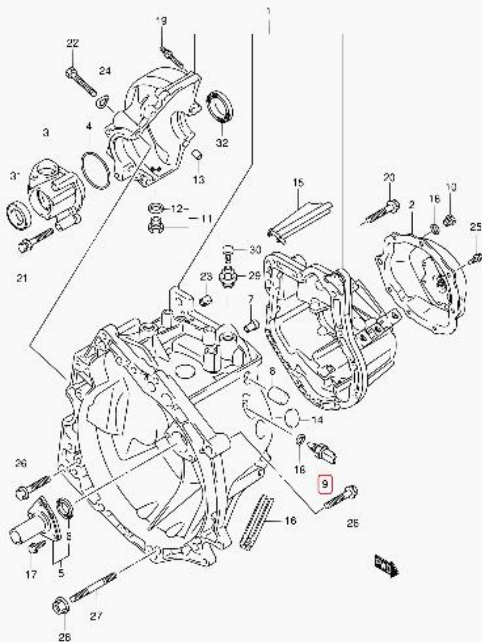
RH416-4 E22 069 MT TRANSMISSION CASE (MT:2WD:DIESEL)
