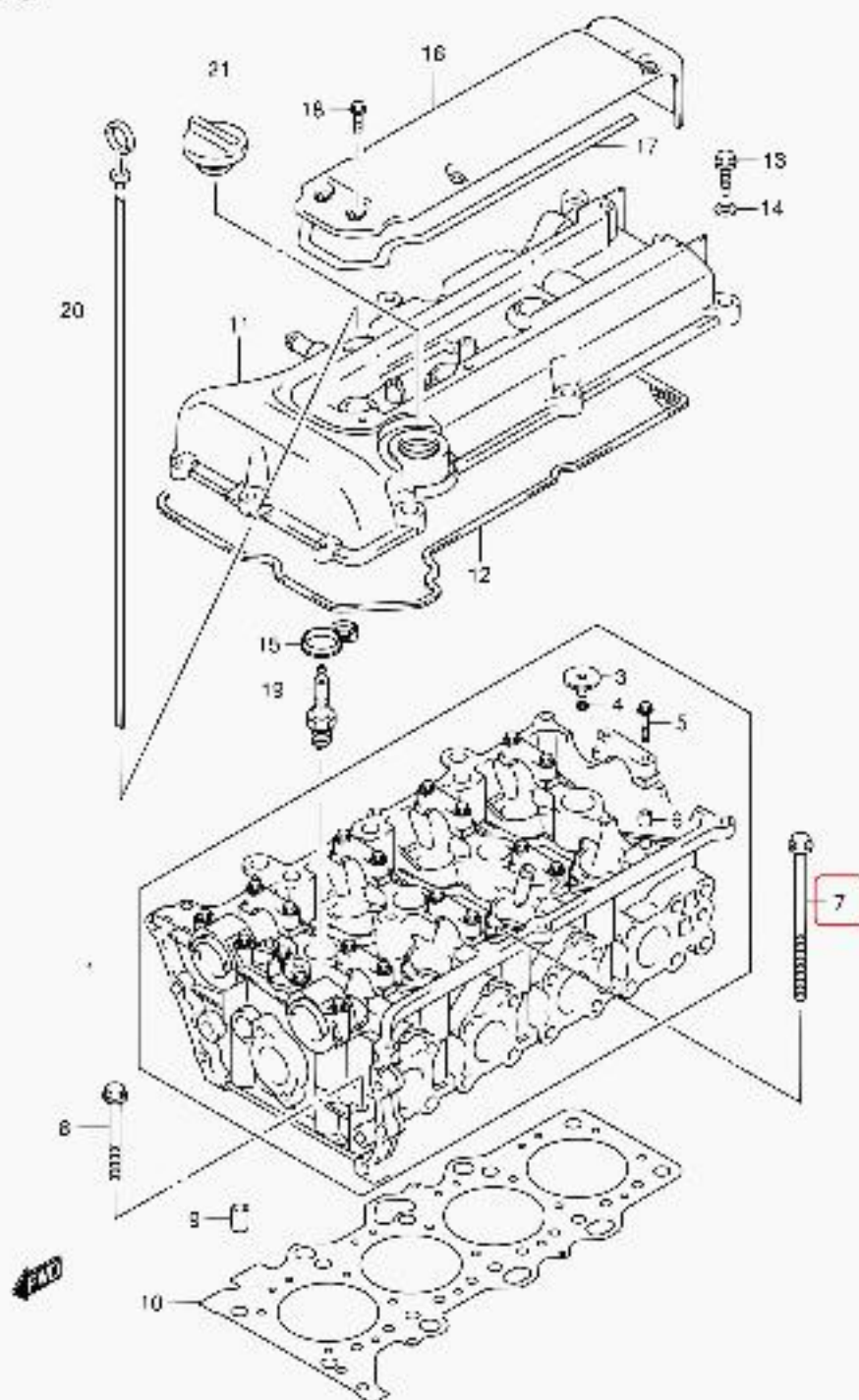
SN413V-2 E22 003 CYLINDER HEAD (SN413V)
