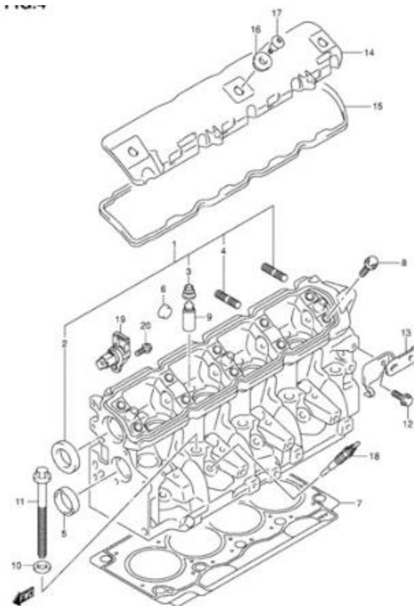
JB420W E22_004 CYLINDER HEAD (JB419)
