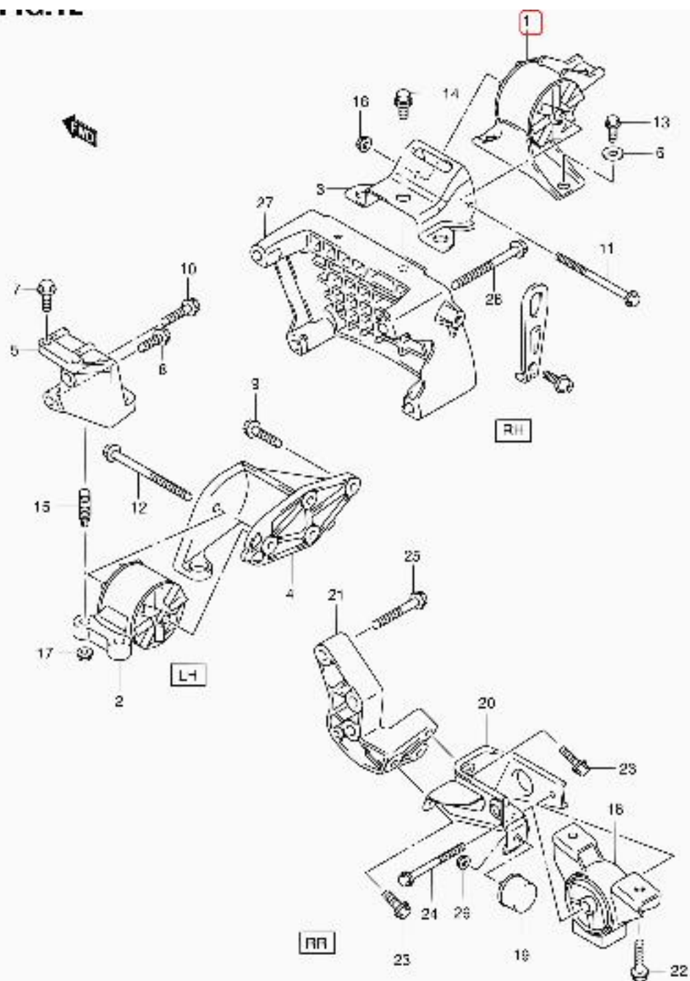
RM413 E22 012 ENGINE MOUNTING (RM413D)
