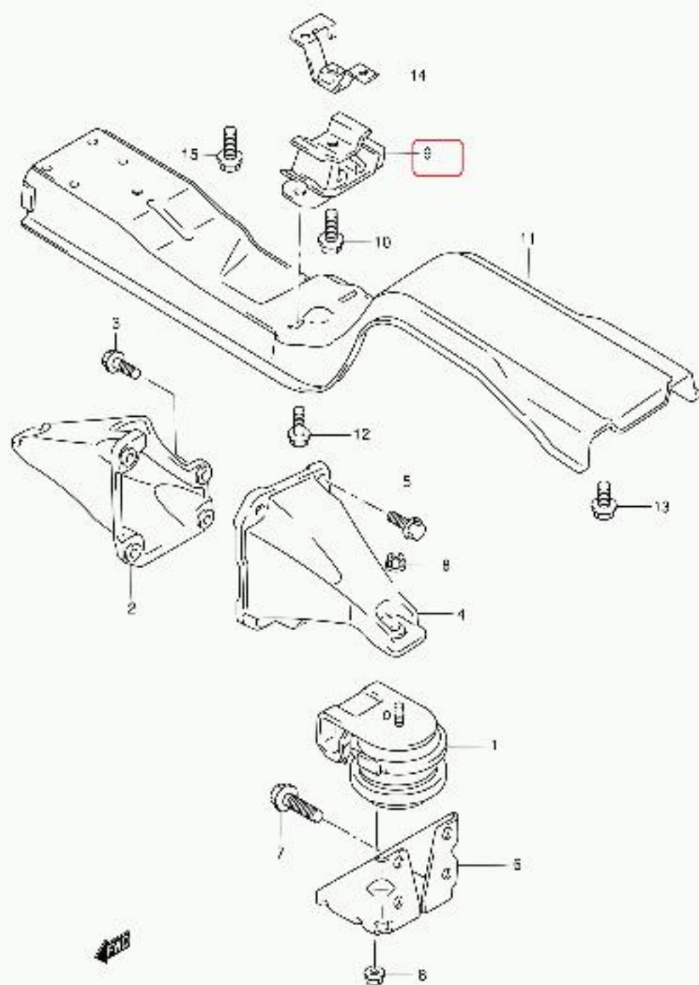
SQ416V-3 E22 012 ENGINE MOUNTING (SQ416/MT)
