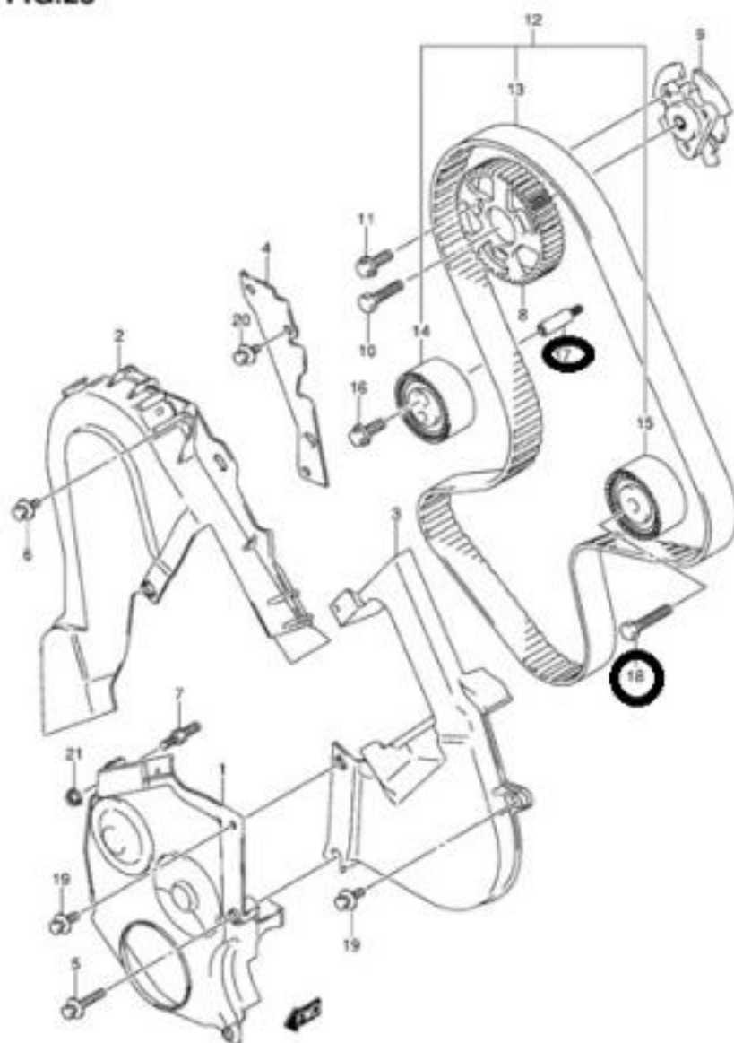
SQ420W-3 E22_023 TIMING BELT (SQ420WD)
