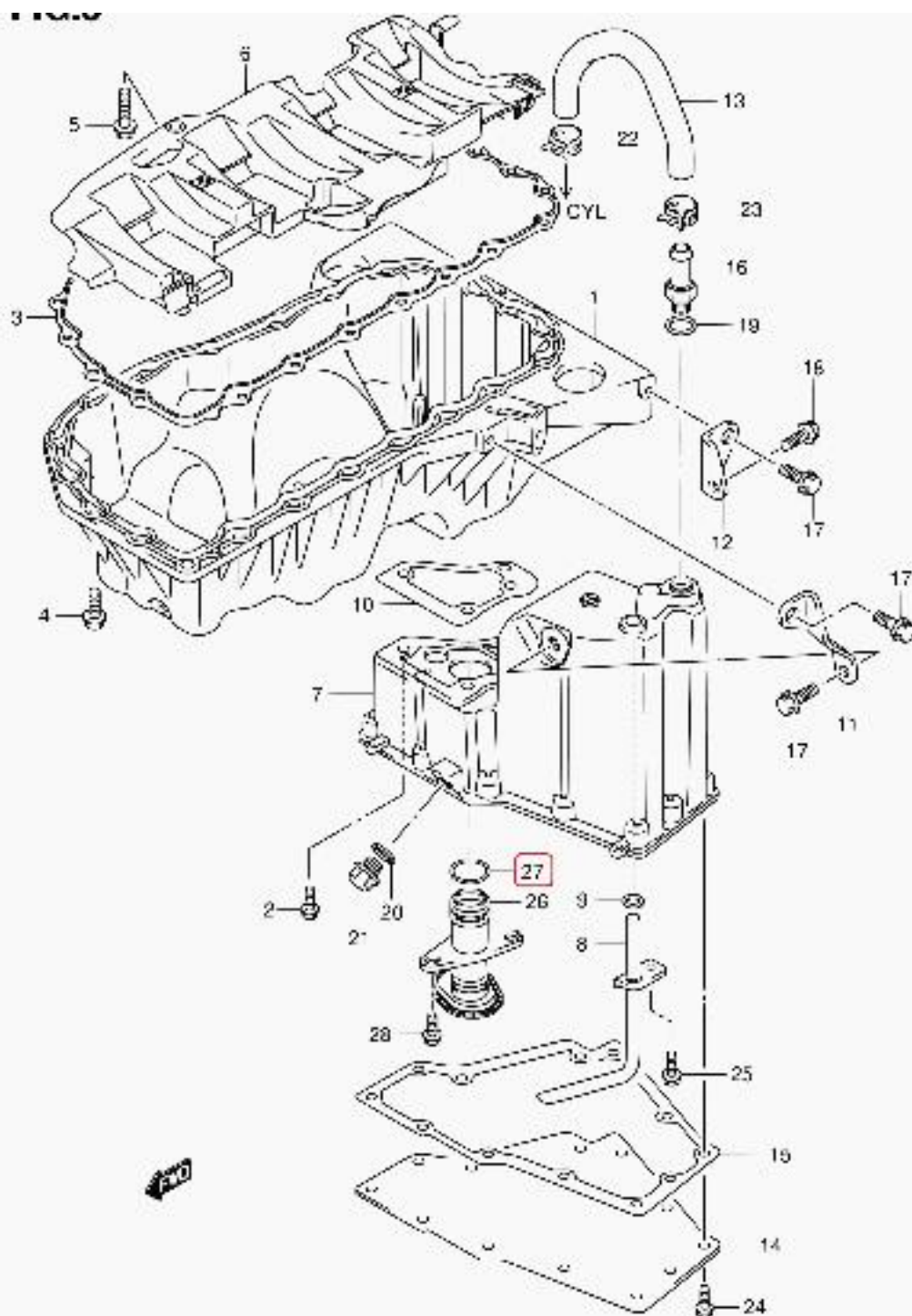
JB420W E22 008 OIL PAN (JB419)
