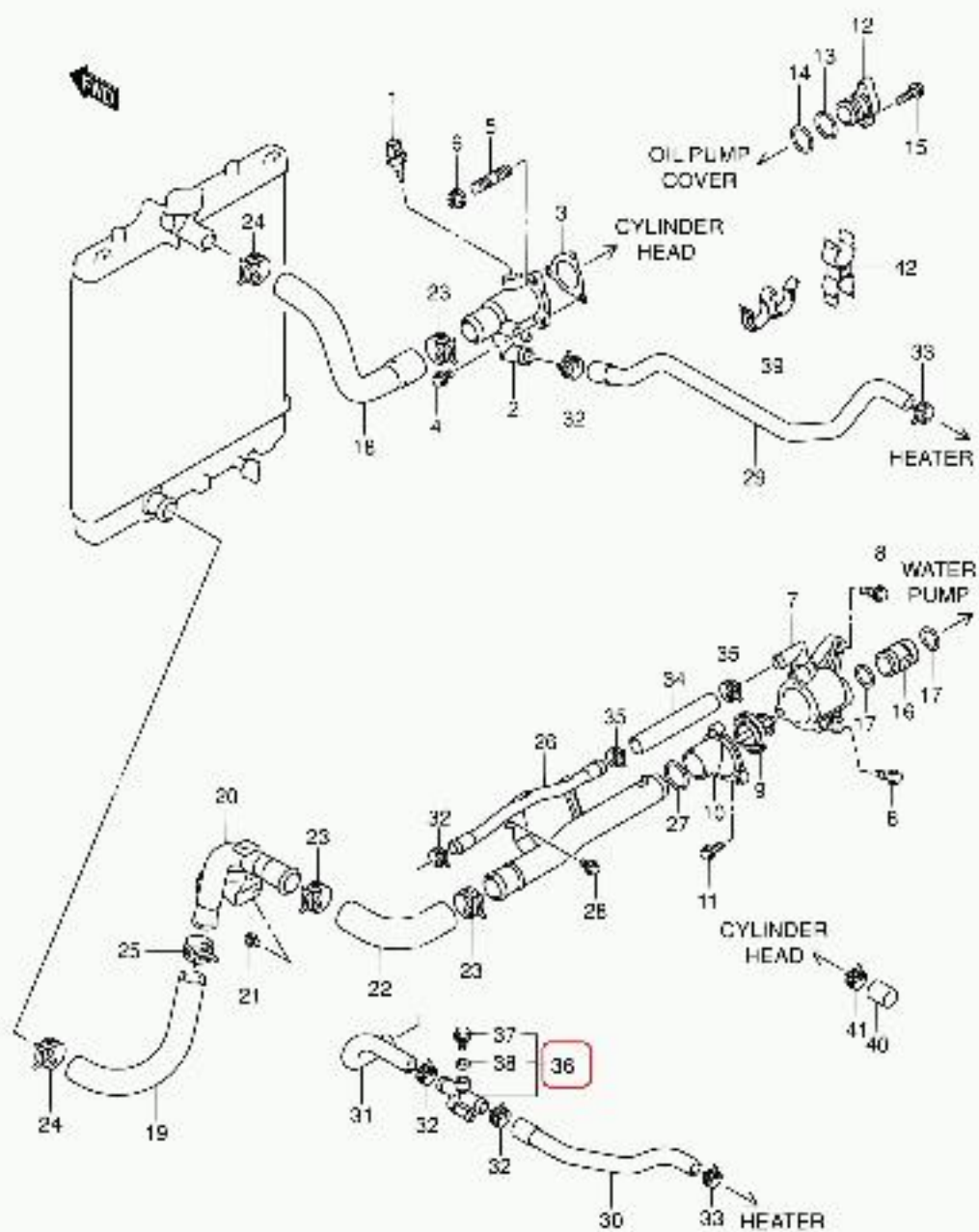
RM413 E22 045 WATER HOSE (RM413 RM415)
