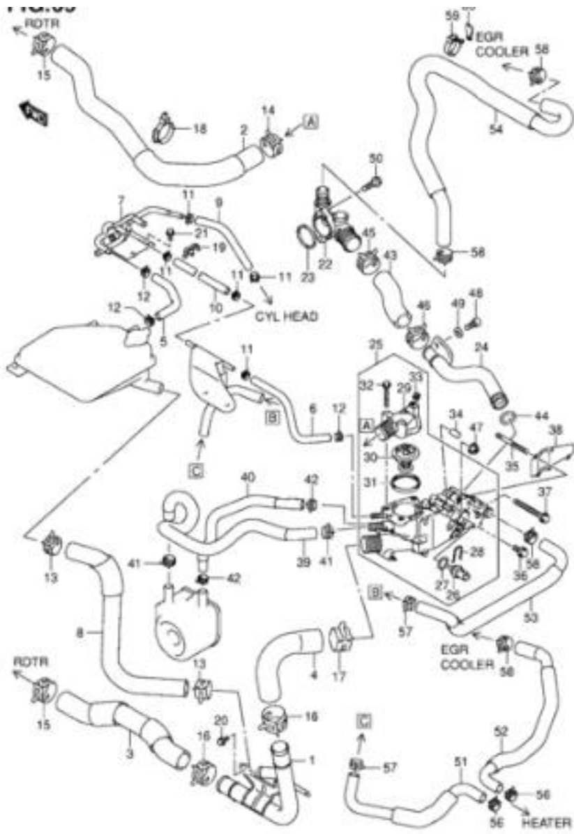
SQ416V-3 E22_069 WATER HOSE (SQ420XD)
