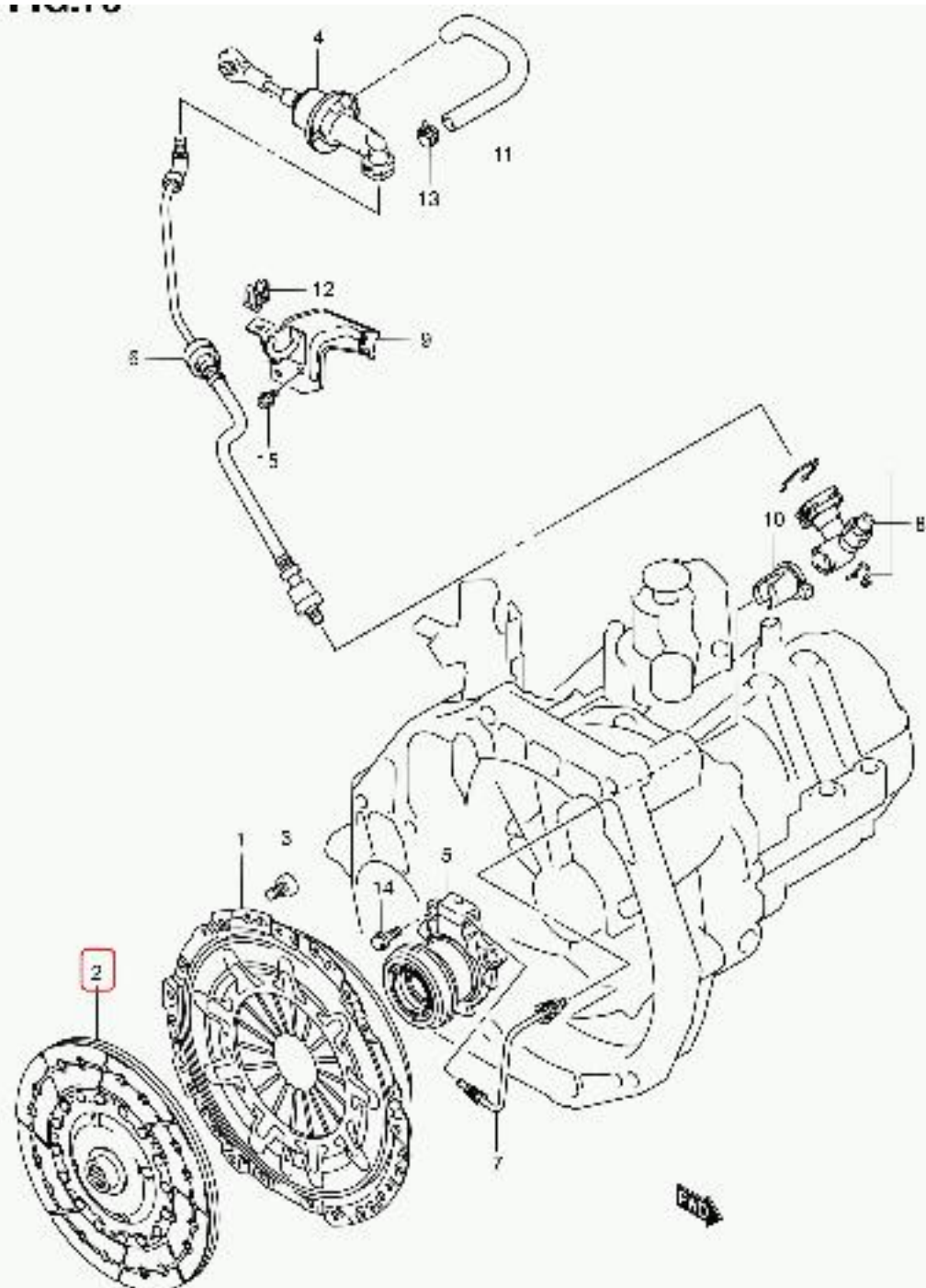
RS413-3 E22 073 MT CLUTCH CONTROL (3)
