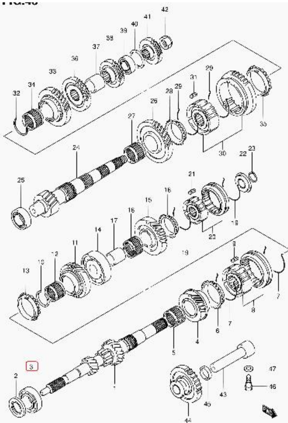
HB413-3 E02 E22 C43 MT TRANSMISSION (HB310:MT)
