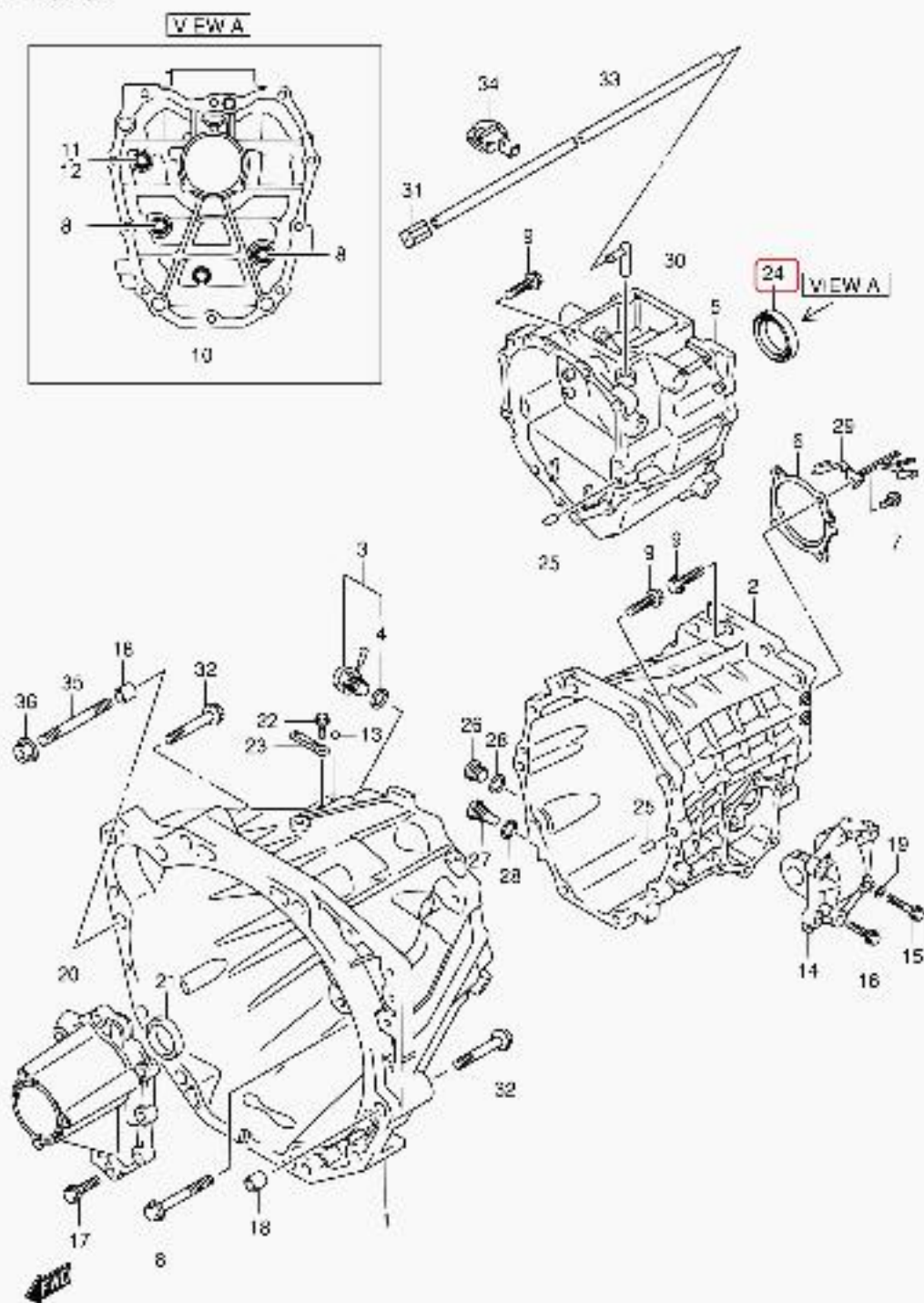
JB420W-4 E22 09/7 MT TRANSMISSION CASE (3)
