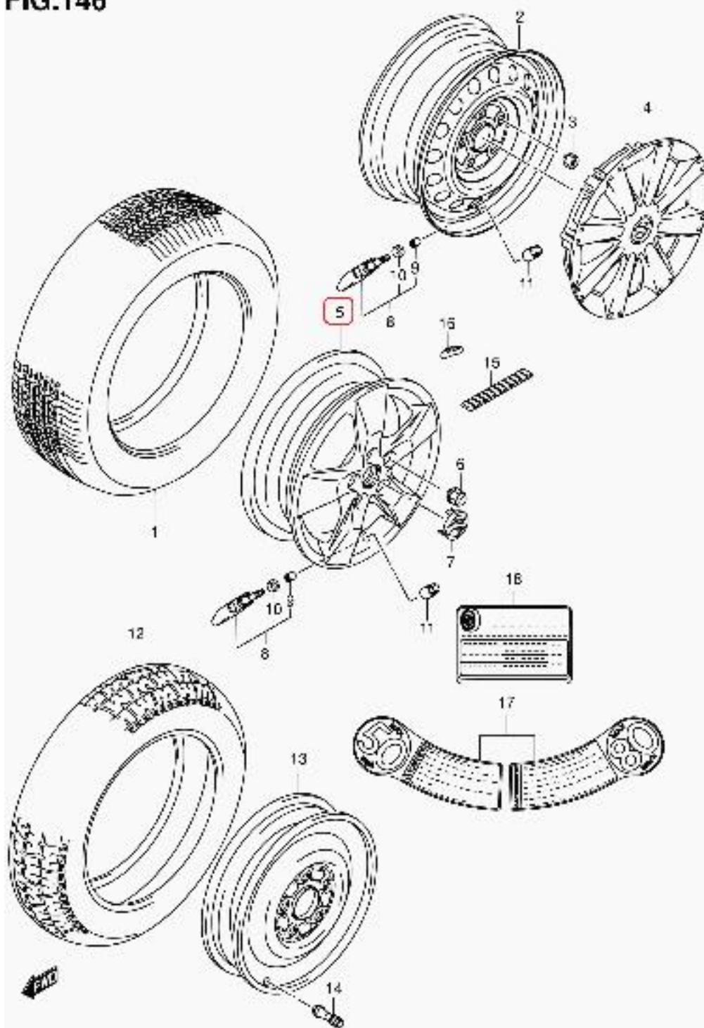
RW120 E60 115 ROAD WHEEL/TIRE (3)
