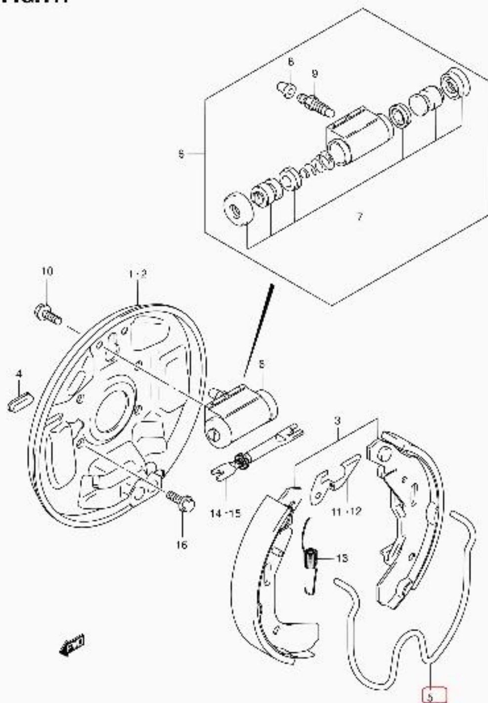
RB413-3 E02 E22 117 REAR WHEEL BRAKE
