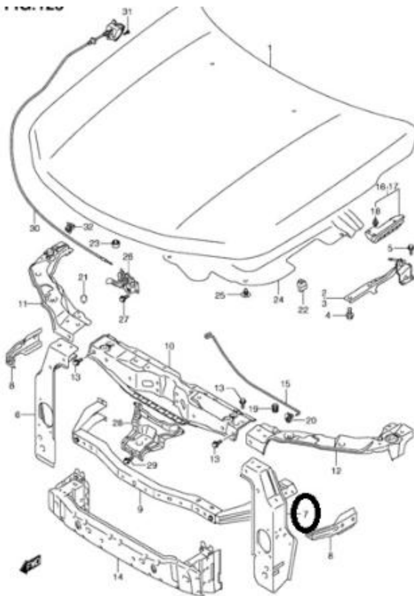
JB424W JB632W E06_125 FRONT HOOD PANEL
