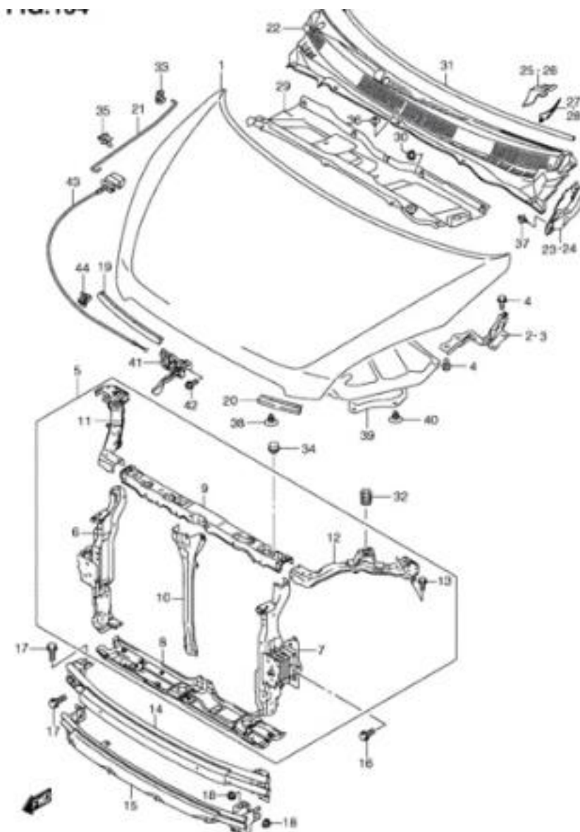
ASB310 E22_154 FRONT HOOD PANEL
