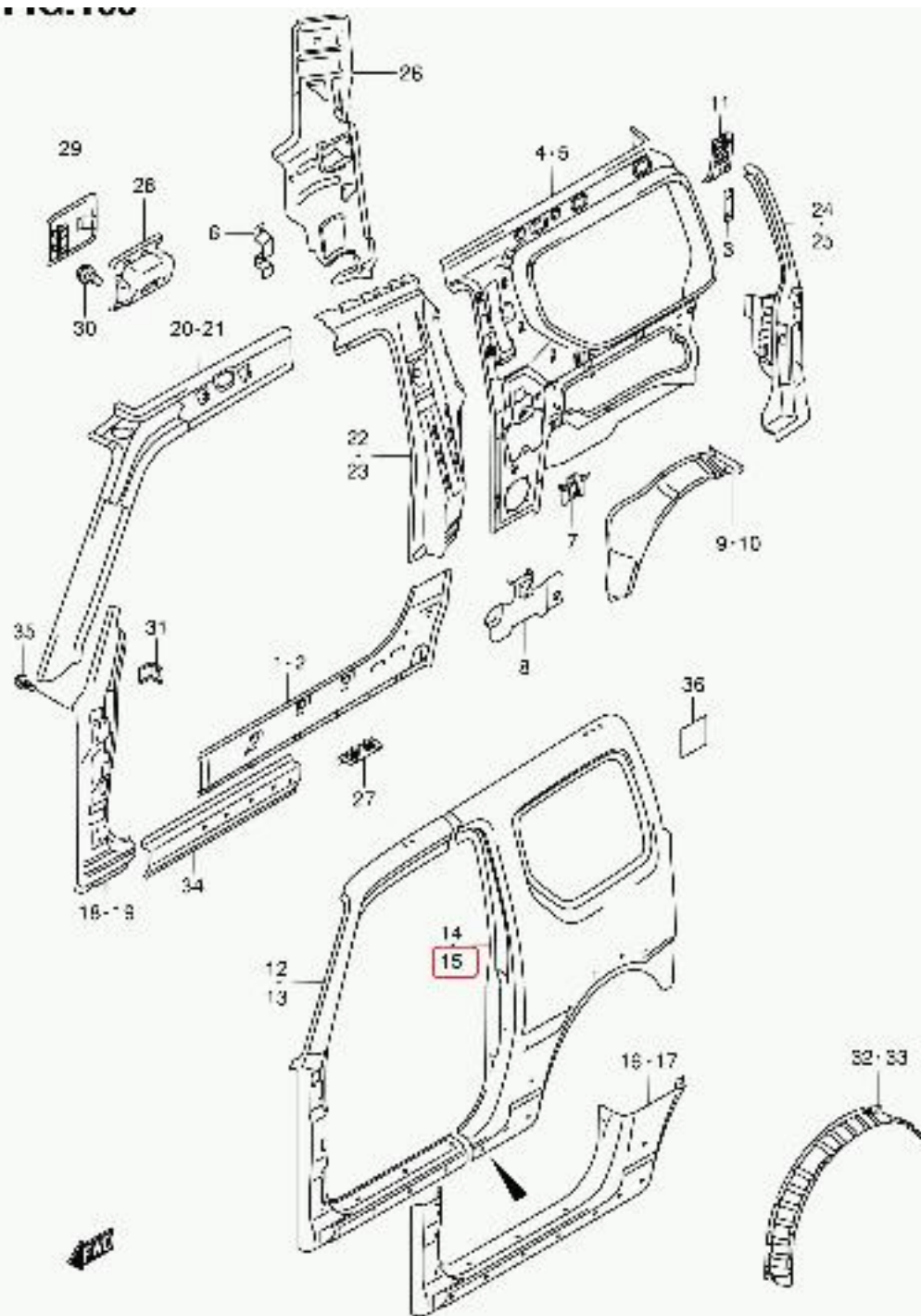
SN413V-2 E22 168 SIDE BODY PANEL
