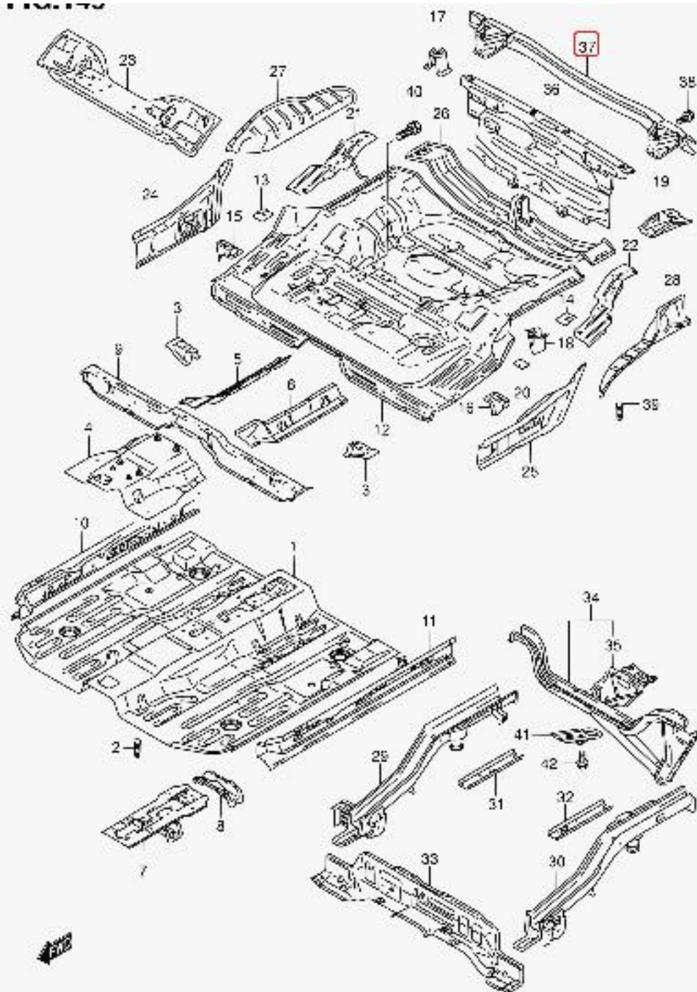
RM413 E22 149 FLOOR PANEL
