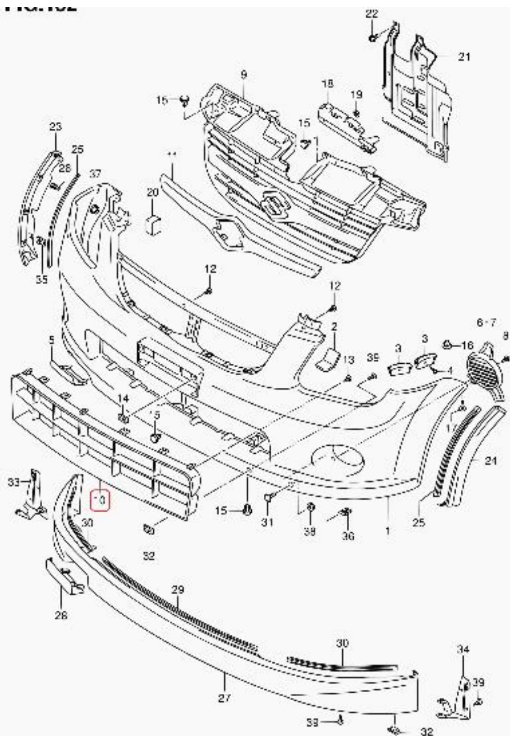
RM413 E22 152 FRONT BUMPER
