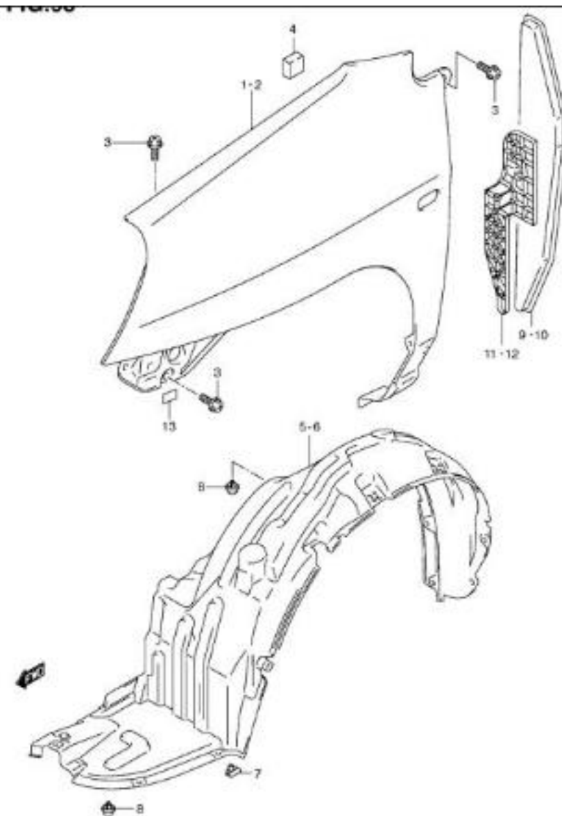
RH423 E60_000 FRONT FENDER
