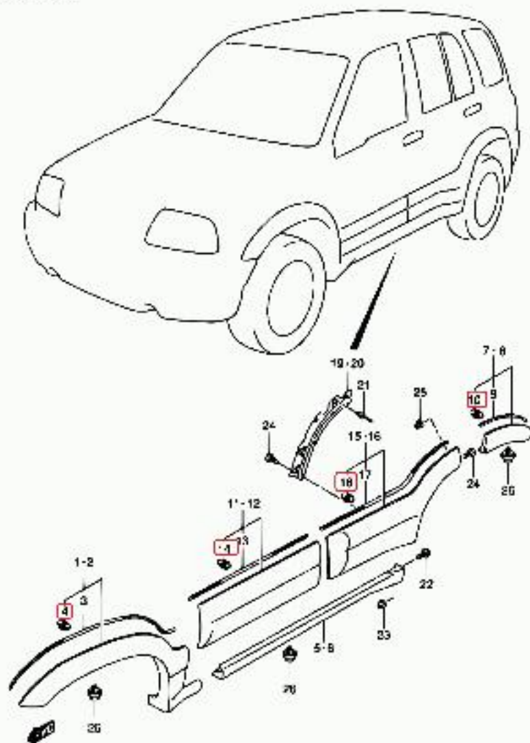
SO42DW-2 E22 253 SPLASH GUARD
