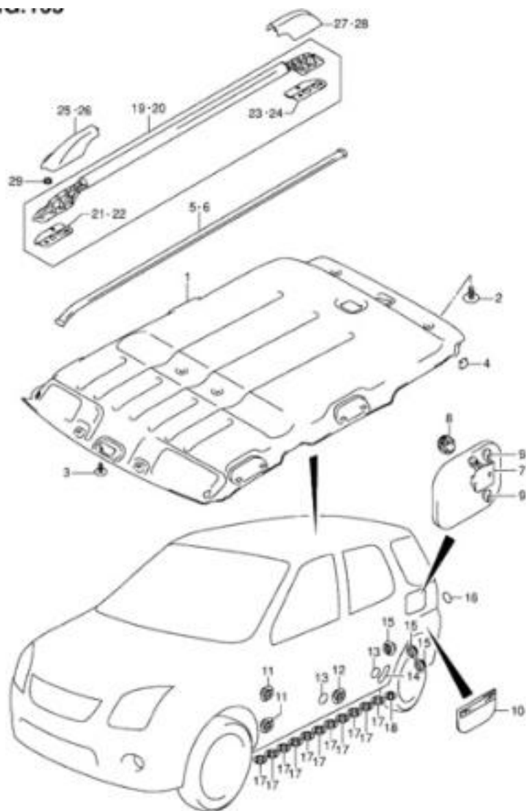
RM413 E22_165 ROOF LINING MOLDING
