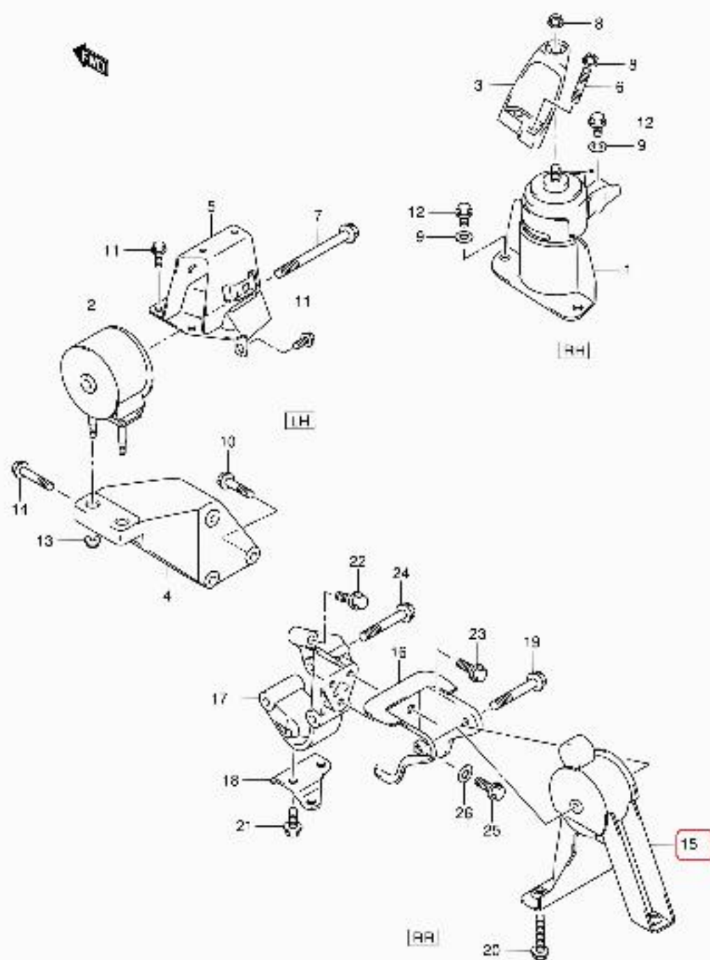
RS413 E22 014 ENGINE MOUNTING (RS413:1)
