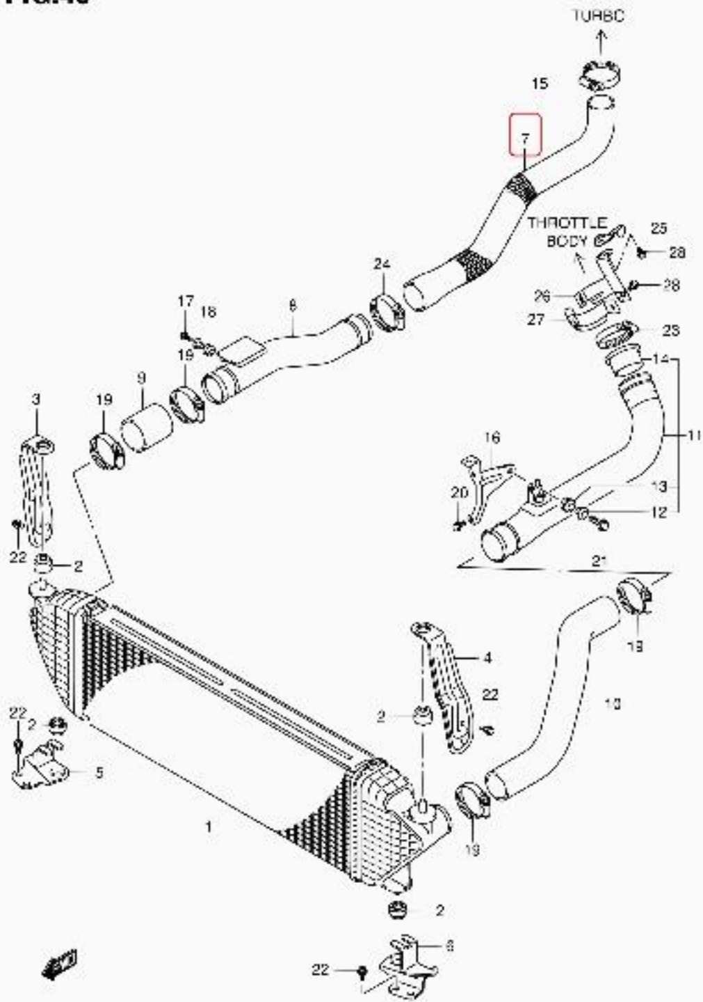
JB415X-4 E22 040 INTER COOLER (1)
