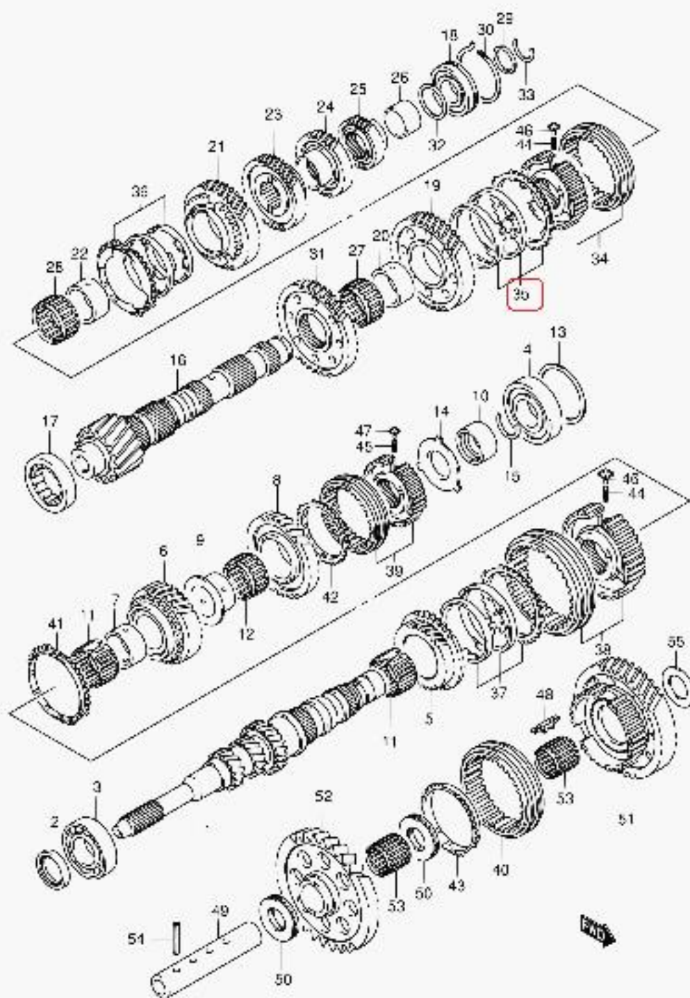
RW418 E22 140 MT TRANSMISSION GEAR (1)
