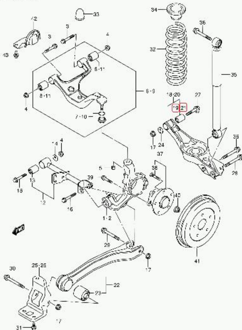
JB420W E22 110 REAR SUSPENSION
