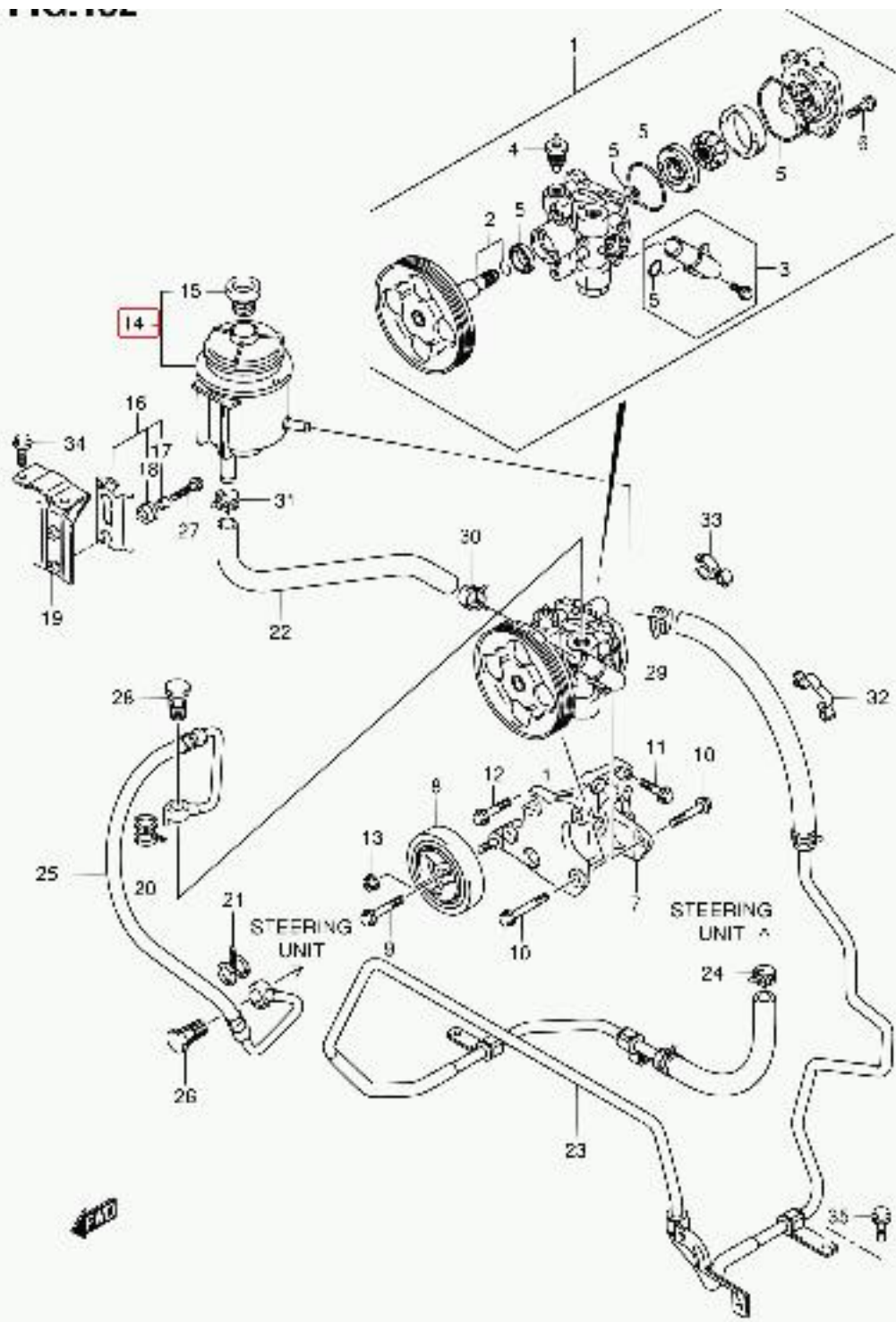
JB416X-4 E22 152 POWER STEERING OIL PUMP (1)
