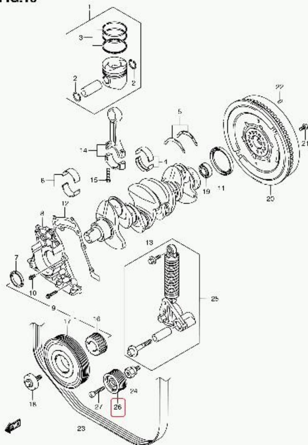
JB116X-4 E22_01 8 CRANKSHAFT (3)
