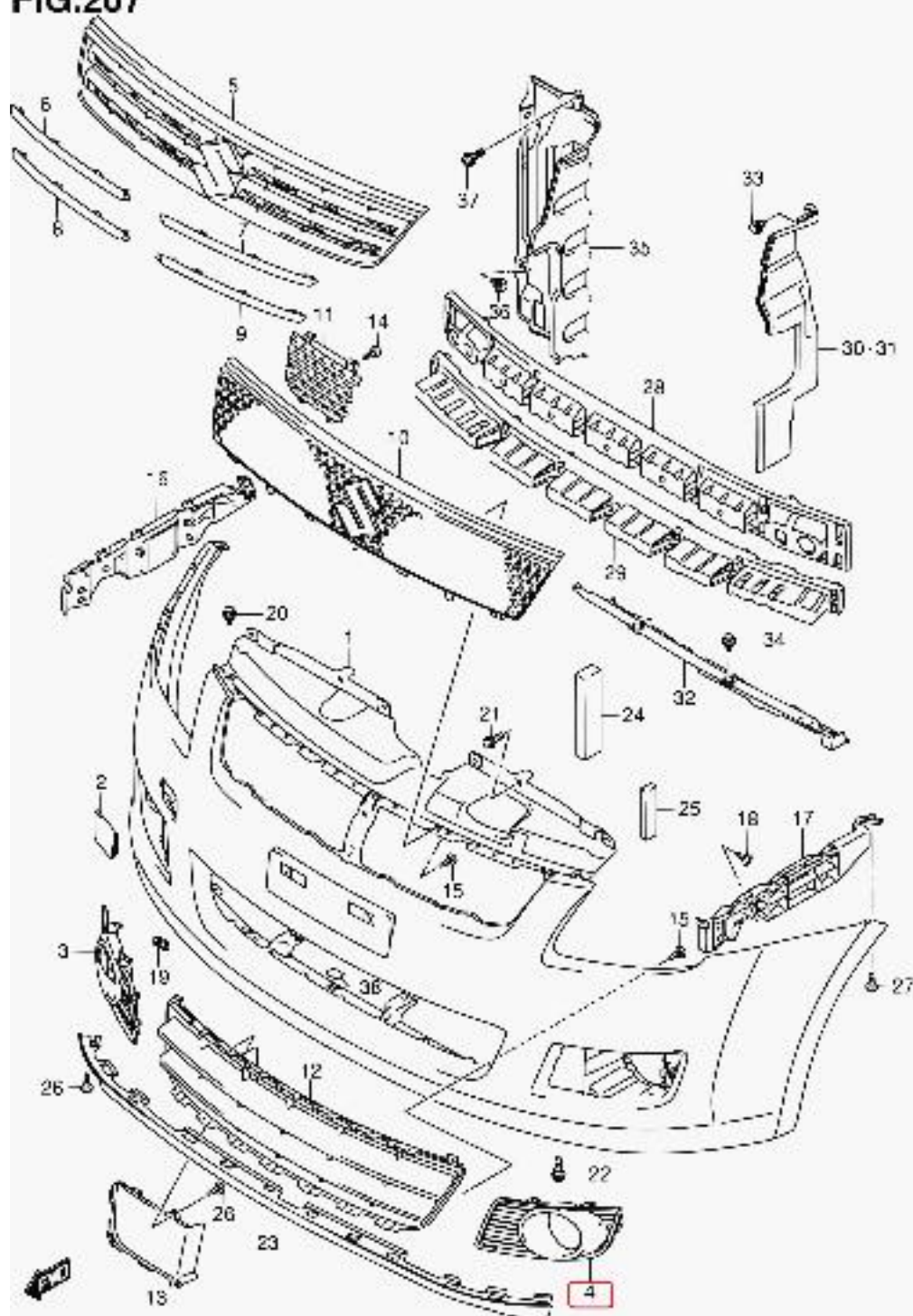
RS413-3 E22 207 FRONT BUMPER (1)
