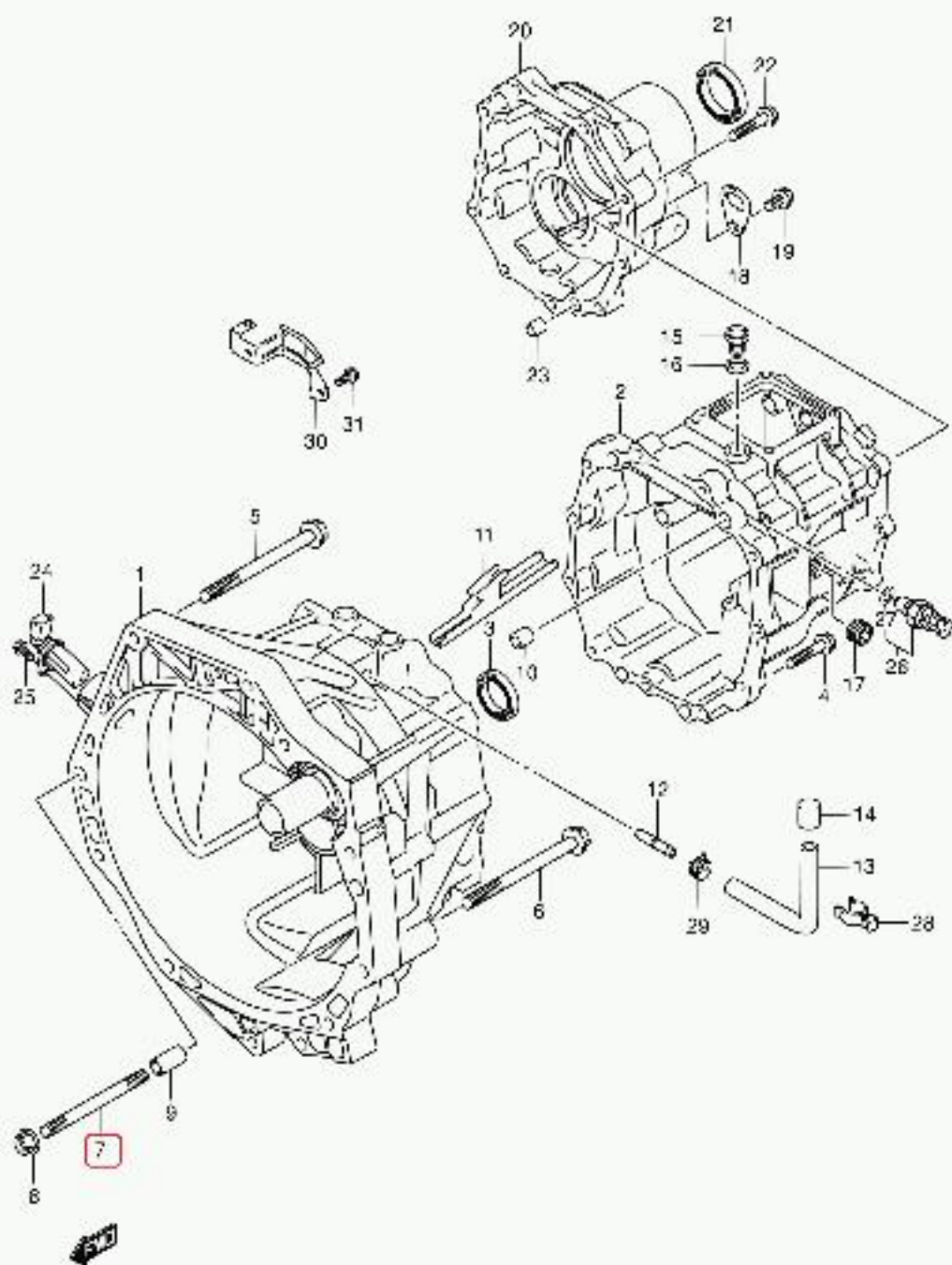
SA413V-5 E22 058A MT TRANSMISSION CASE (3)
