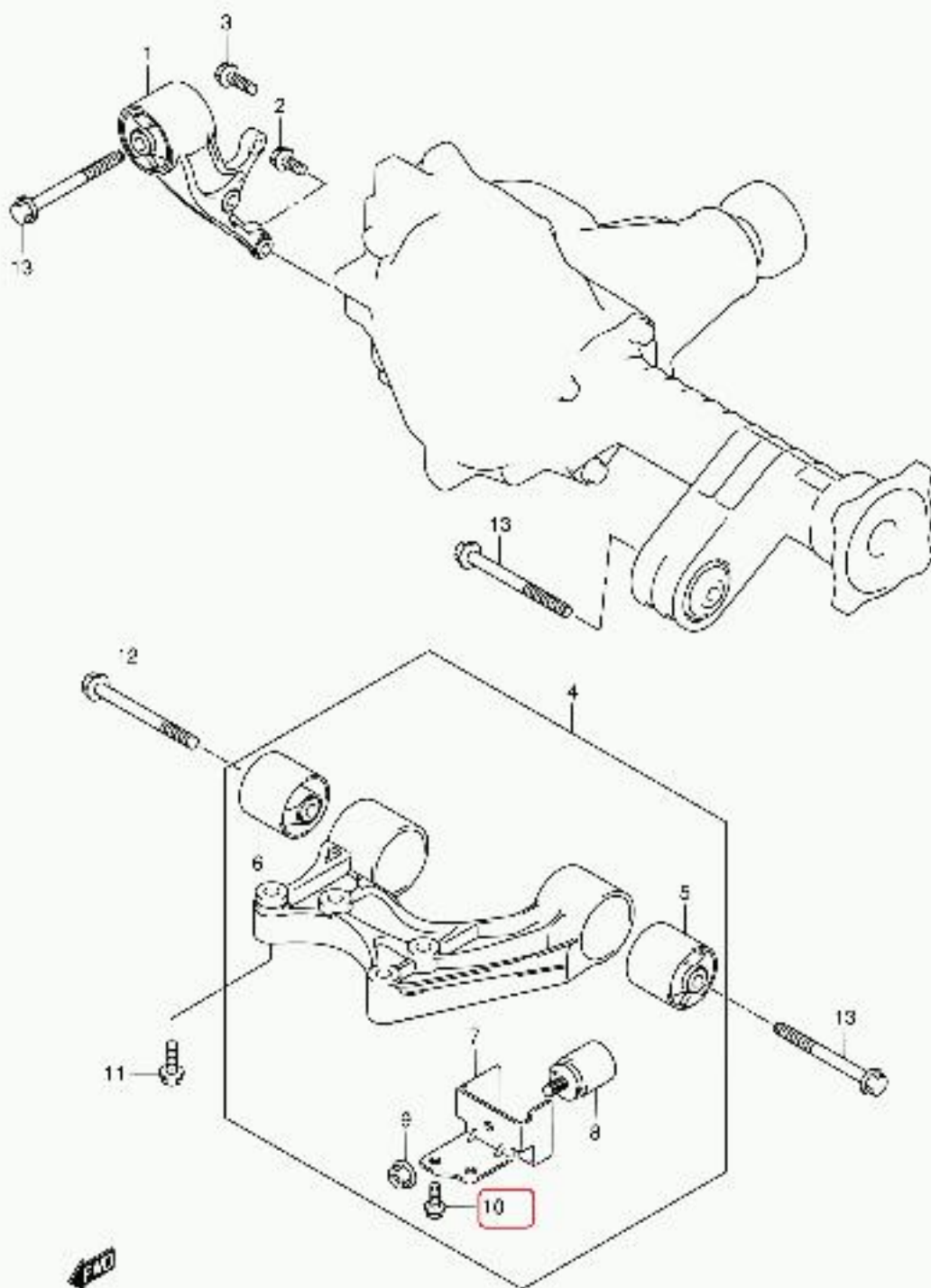
J3627W E21 015 FRONT DIFF MOUNTING (4WD:1)
