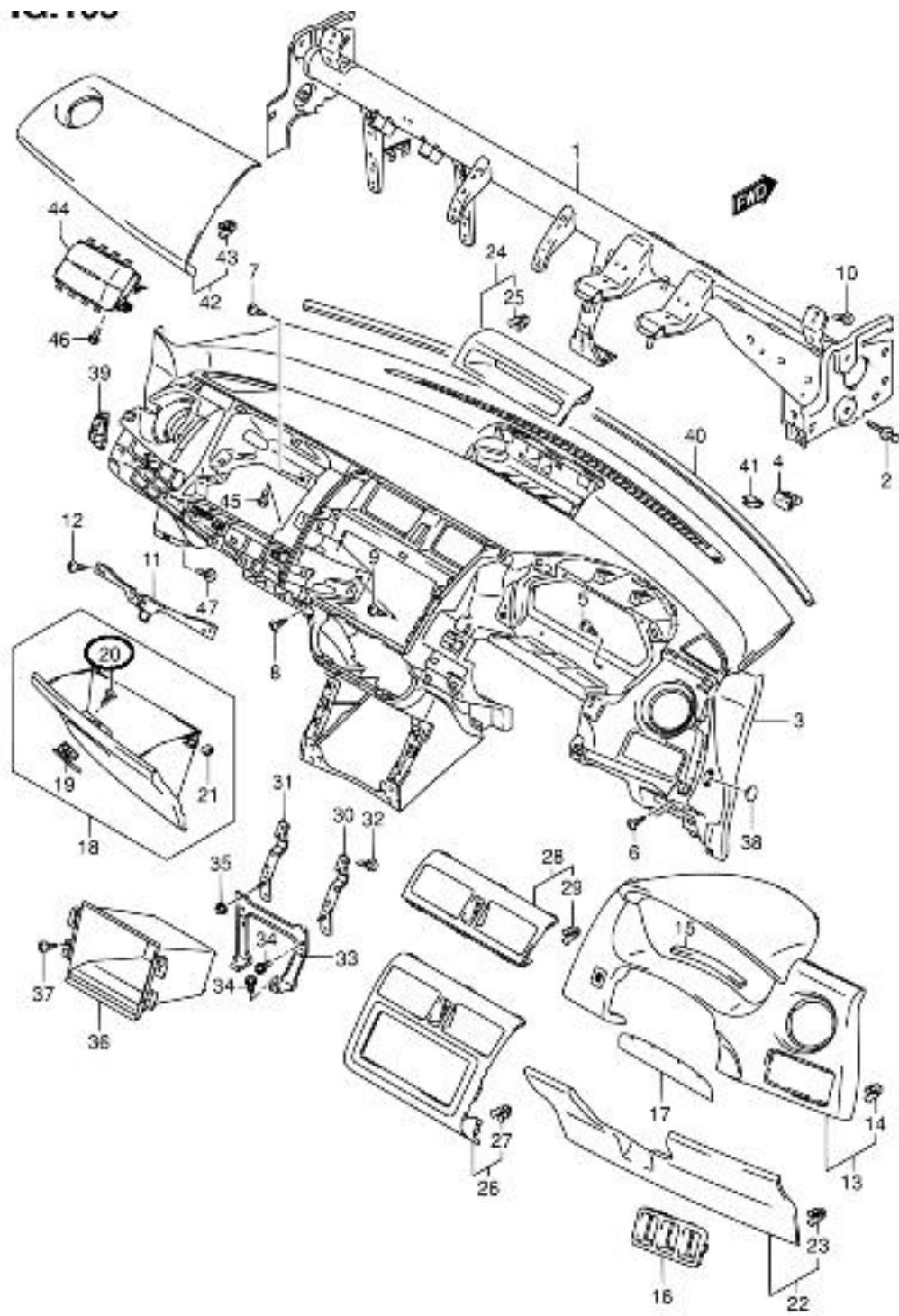
RS415 E24 165 INSTRUMENT PANEL (2)
