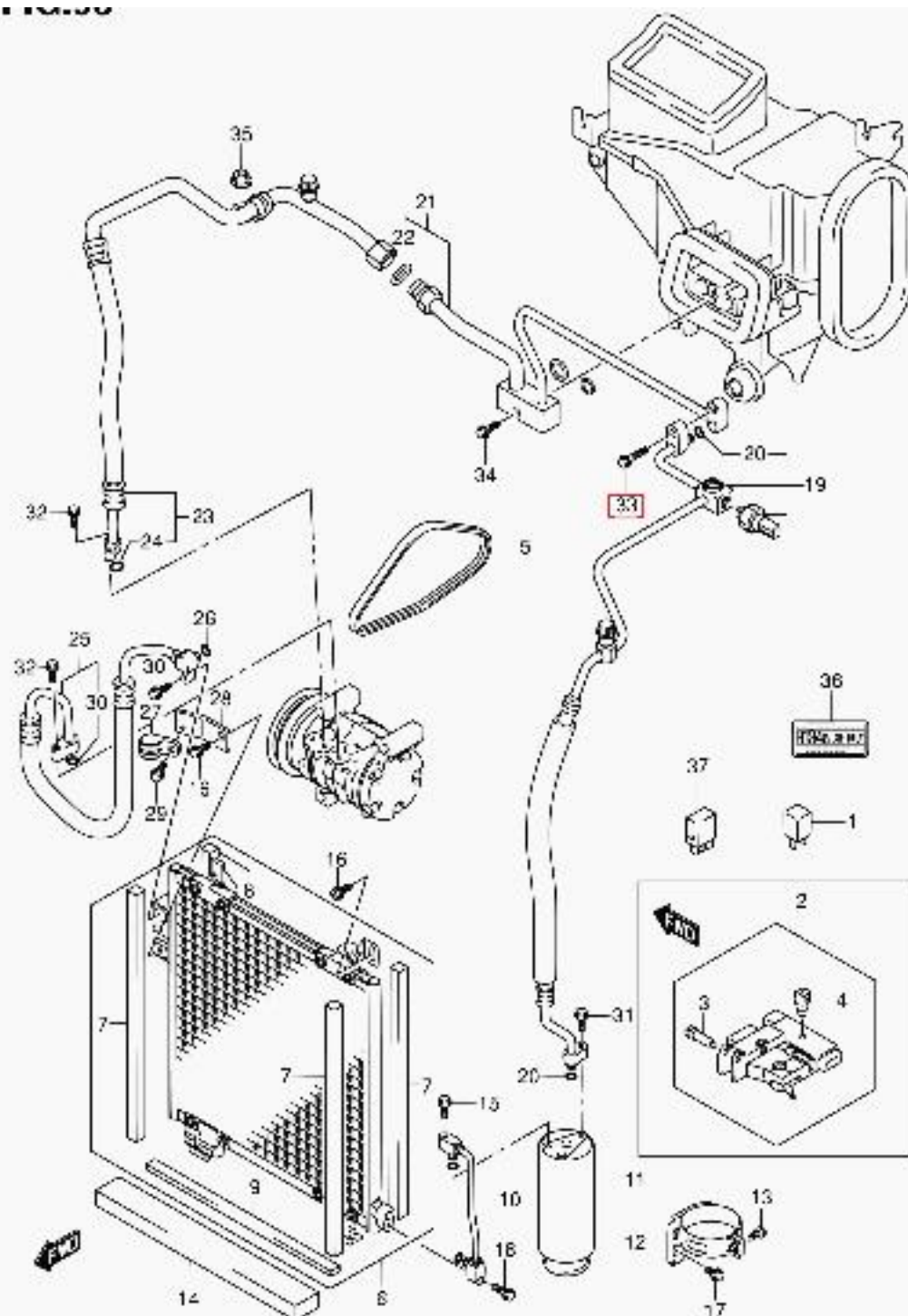
RF410 P/O P43 093 AIR CONDITIONER
