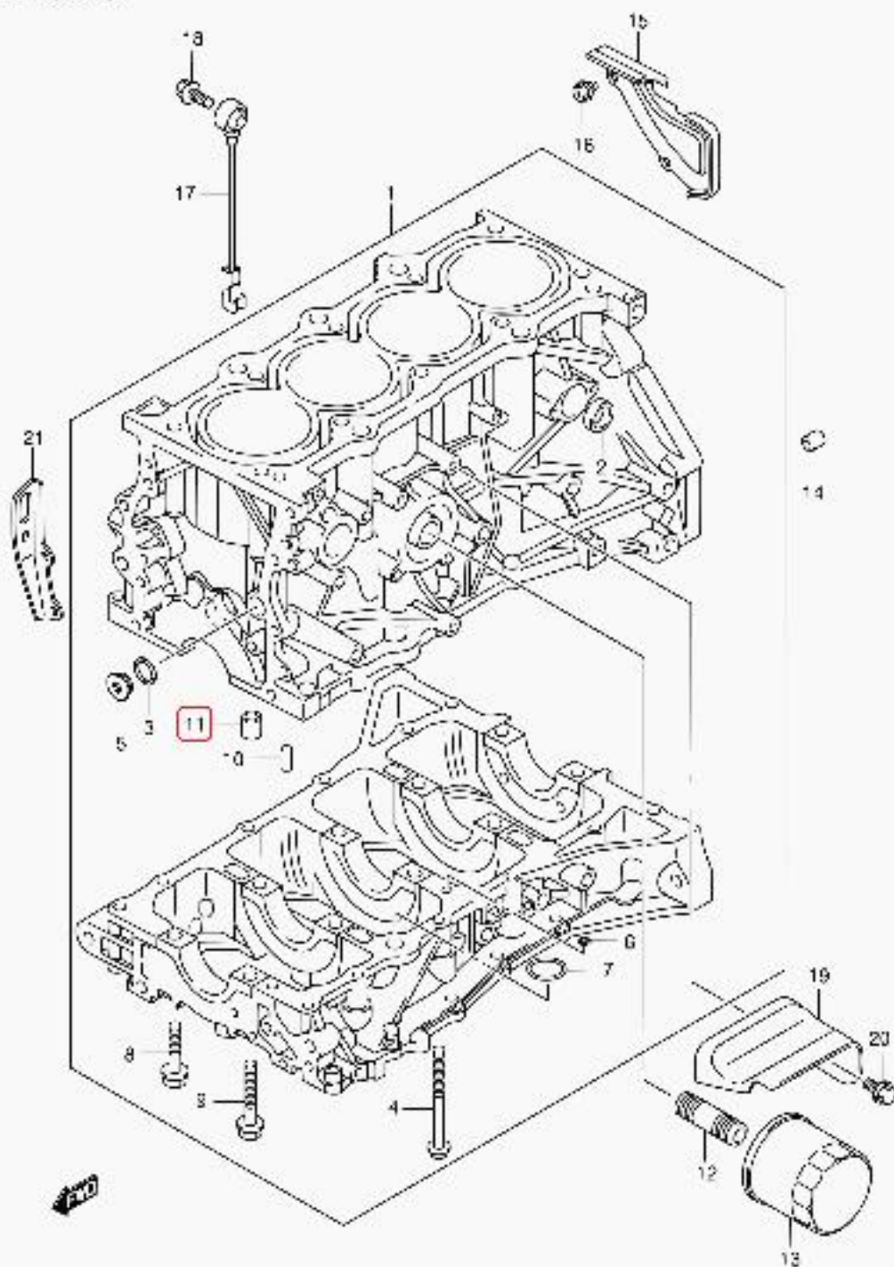
JB420W-4 E22 010 CYLINDER (2)
