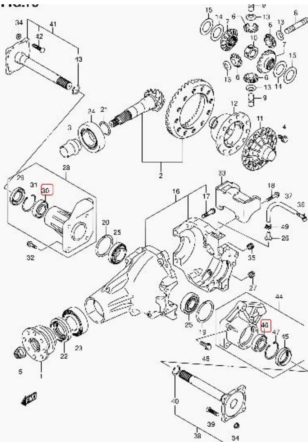
JB420W E22 075 REAR DIFF GEAR
