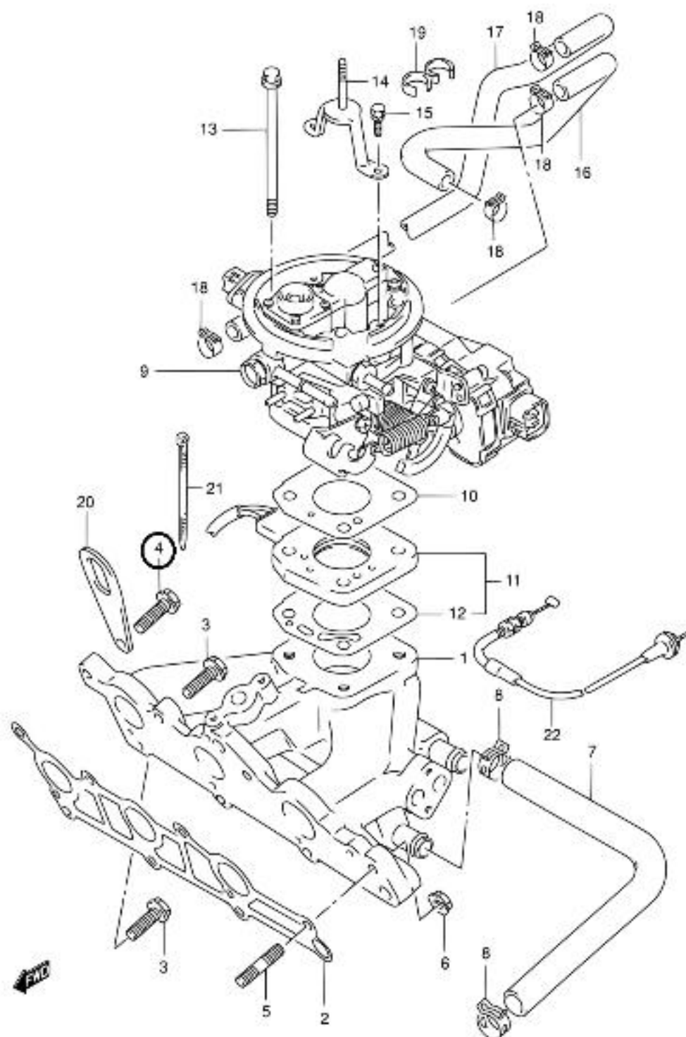
SF416-2 E66 027A INTAKE MANIFOLD&THROTTLE BODY(SF310)
