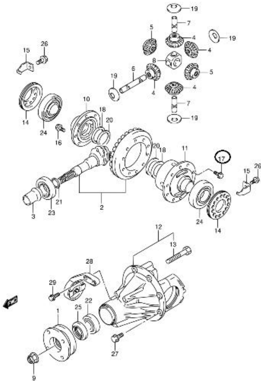
SN413V-5 E22 078 REAR DIFF GEAR
