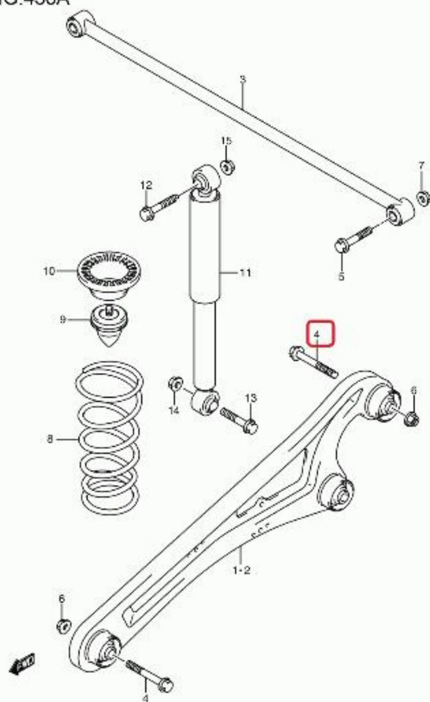
DA64V5Y_430A REAR SUSPENSION
