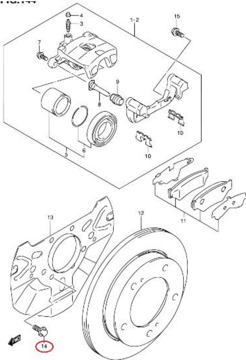
SN413V-5 E22 144 FRONT WHEEL BRAKE (2)
