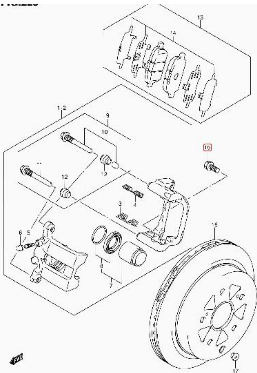
JB420W-4 E22 220 REAR WHEEL BRAKE
