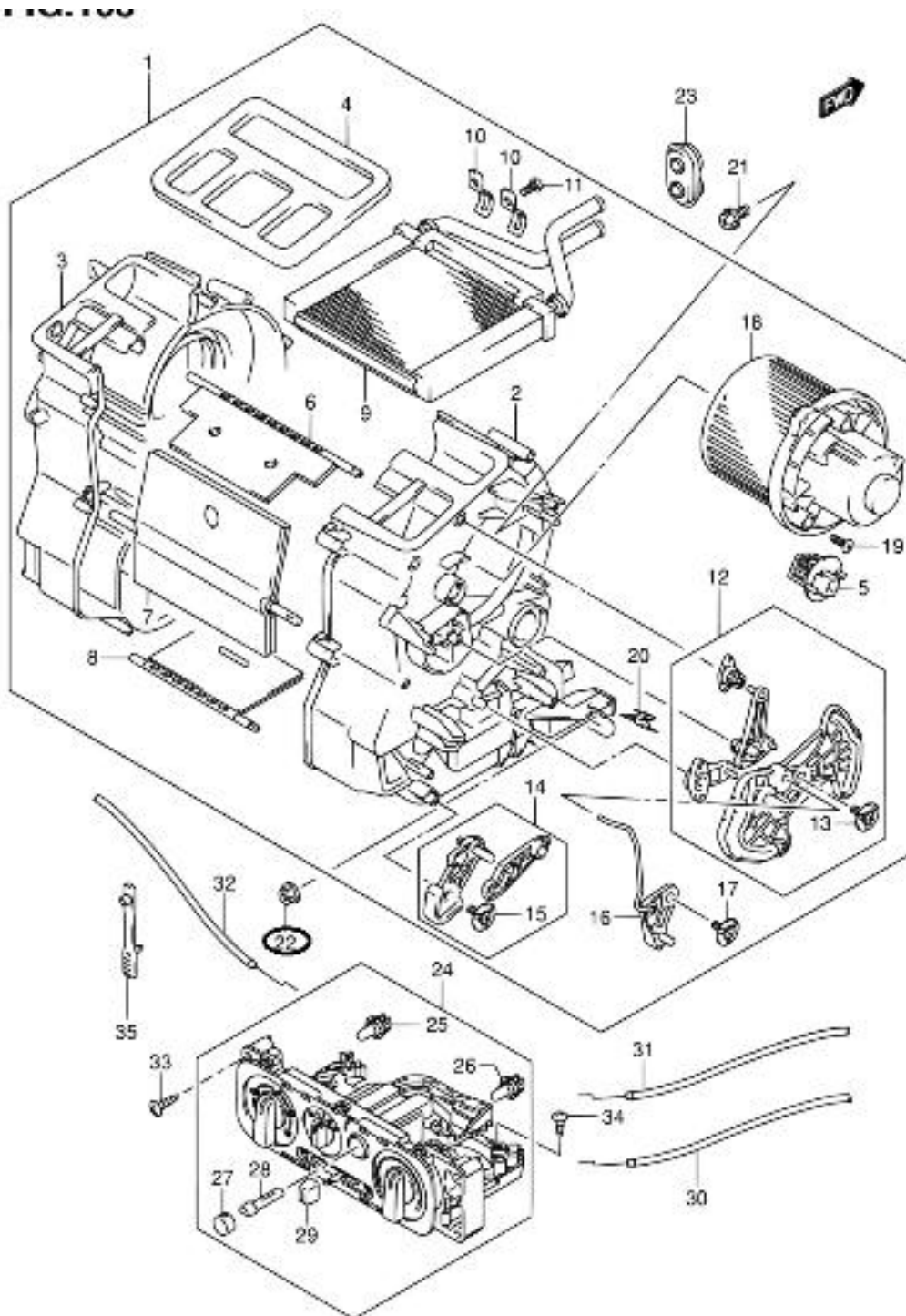
SN413V-5 E22 163 HEATER UNIT (2)
