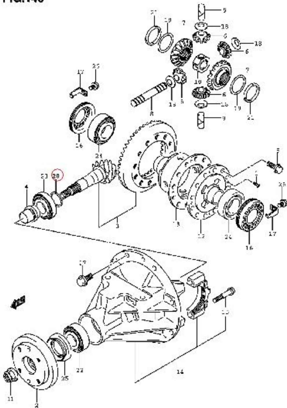
SQ421W-2 E23_146 REAR DIFF GEAR (SQ421WD::RHS-MT)
