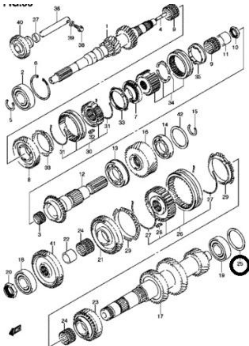
BN413V-5 E22_058 MT TRANSMISSION GEAR (2)
