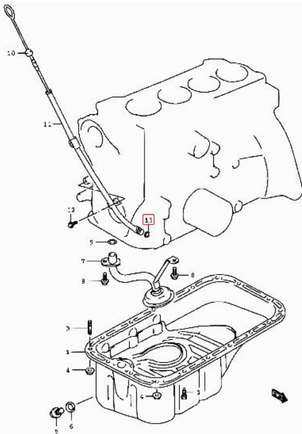
SY413-7 E01_010 OIL PAN (SY416)
