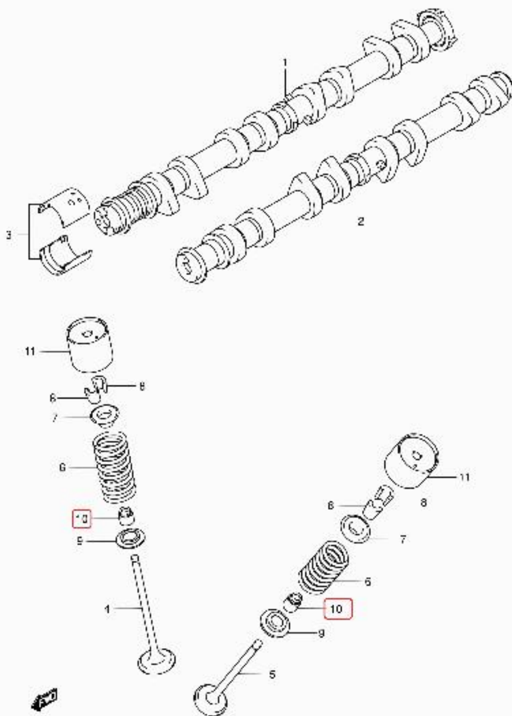
JB420W-4 E22 025 CAMSHAFT/VALVE (2)
