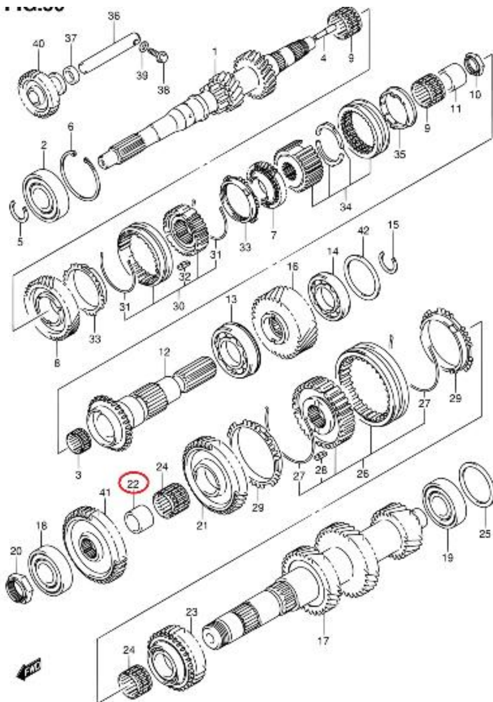
SN413V-5 E22 056 MT TRANSMISSION GEAR (2)
