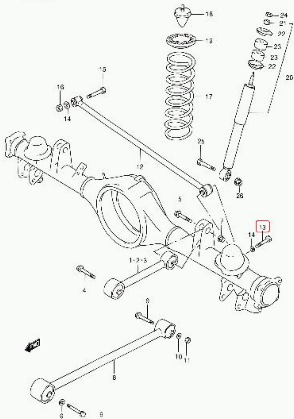
SQ420Q E22_098 REAR SUSPENSION
