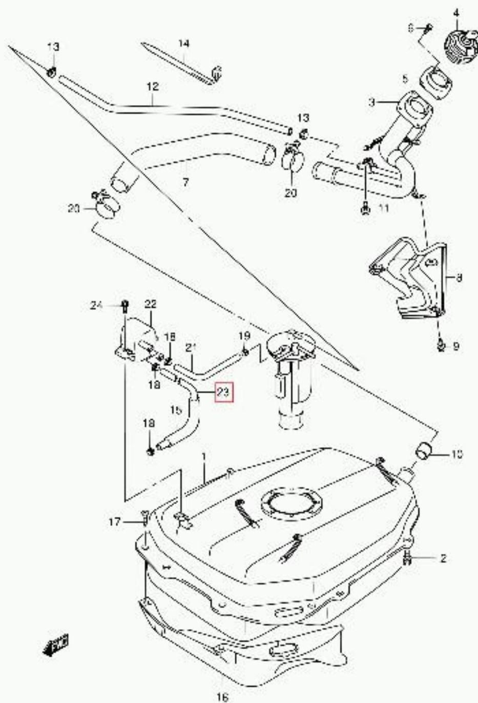
RB413-3 E02 E22 160 FUEL TANK
