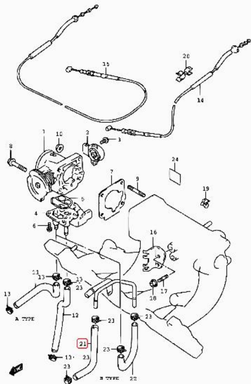
SY413-7 E01_027 THROTTLE BODY (SY413, SY416)
