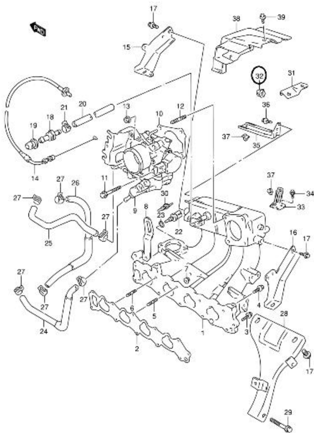
SZ416 E01 011A INTAKE MANIFOLD/THROTTLE BODY (2)
